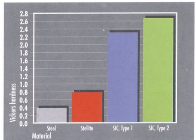
Wear of nozzle materials
