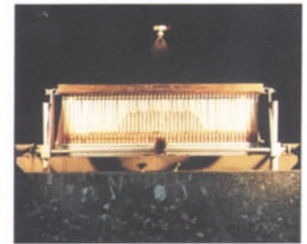
A line of measurements flasks with electronic evaluation for measurement of liquid distribution
