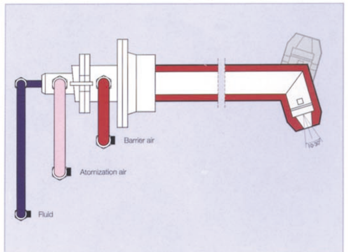
A twin-fluid supersonic nozzle with barrier air
