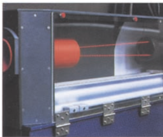
Measurement set-up Laser-Doppler particle analyser
